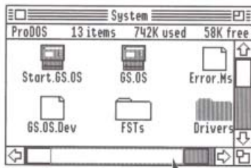
Figure 3-6 Scrolling techniques
