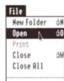
Choose Open
