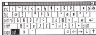
Option characters
