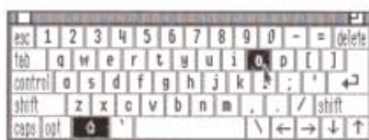
Pressing Command-O
