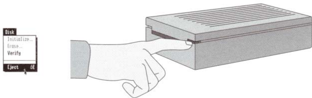
Choosing Eject
